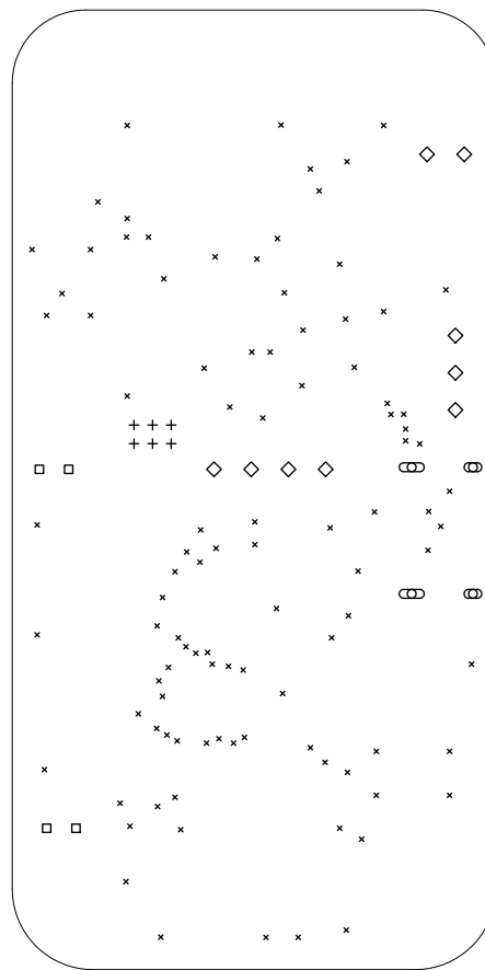
Drill Map:
